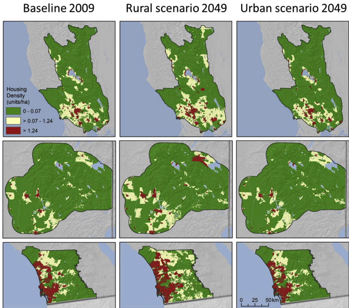
Fig. 4. Classified housing density in 2009, 2049 for the rural, and 2049 for the urban scenarios in the a) North Coast, b) Butte-Plumas, and c) San Diego County study areas. The middle (yellow) class represents the housing density range across the three study areas where structures have been destroyed in the past (For interpretation of the references to colour in this figure legend, the reader is referred to the web version of this article).
