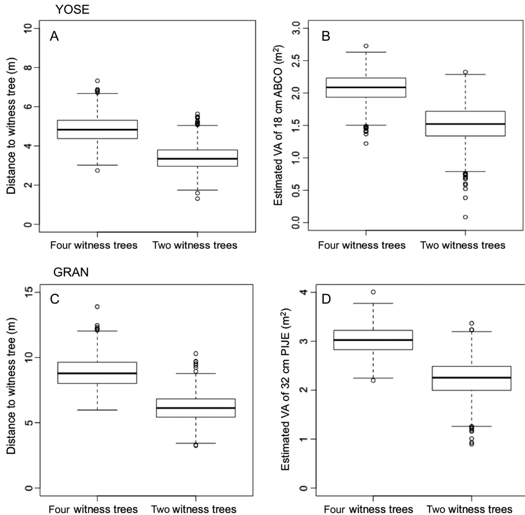
FIG. 3. Simulation results (1000 runs) of the mean neighborhood distance (A, C) when two witness trees or four witness trees are used for a six-point sampling scheme for the YOSE and GRAN sites, respectively. The discrepancy in mean neighborhood distance is reflected in the estimate of the Voronoi area of a single tree of the dominant species (B, D) of the median DBH in that plot using the method and equation parameters in Baker (2014). Results for other sites are shown in Appendix S1: Fig. S4. ABCO refers to Abies concolor (white fir); PIJE refers to Pinus jeffreyi (Jeffrey pine). The midline of the boxplot represents the median of the data, the upper and lower limits of the box represent the third and first quartile of the data, and the whiskers represent 1.5\times the interquartile range from the third and first quartile. The points represent data outside 1.5\times the interquartile range from the third and first quartile.
