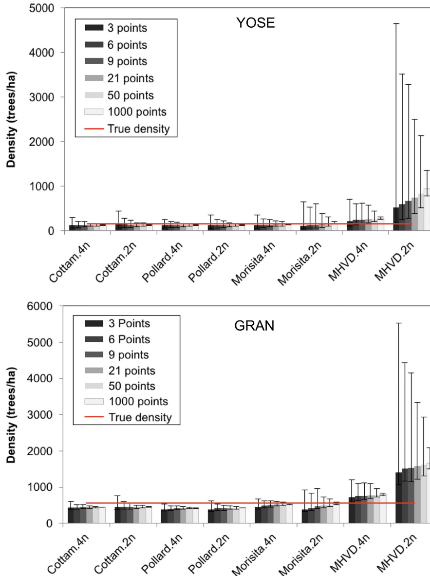
FIG. 2. Results of simulations testing the effect of sampling intensity (number of sampled points) on the Cottam, Pollard, Morisita, and MHVD estimators at the YOSE and GRAN (developed from granitic material) sites. Bars show the median value of 1000 realizations and error bars show the 95% confidence intervals. Simulation summaries can be found in Appendix S1: Tables S1–S9. [Color figure can be viewed at wileyonlinelibrary.com ]
