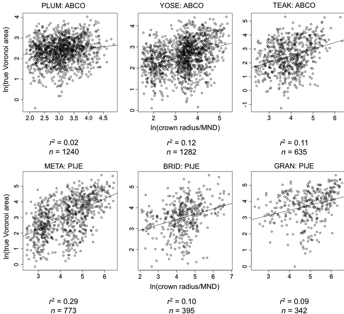
FIG. 4. The relationship of true Voronoi area (VA) to crown radius (CR) for the dominant tree species at each of the six study sites. The crown radius was estimated using parameters for species-specific fits derived from Forest Health Monitoring measurements in Sierra Nevada mixed-conifer plots (PIJE, n = 164 ; ABCO, n = 746 ). MND is the mean neighborhood distance (see Eq. 3). ABCO refers to Abies concolor (white fir); PIJE refers to Pinus jeffreyi (Jeffrey pine).
